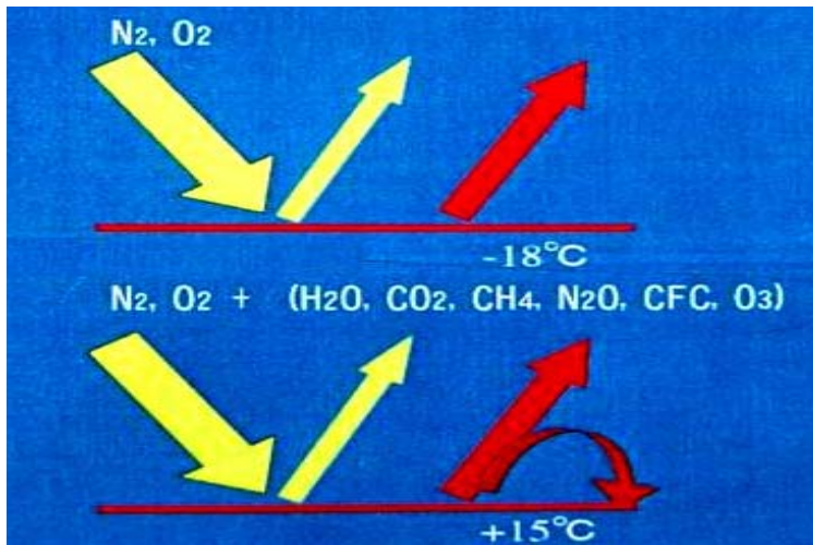
Figure 7.2 Transparent and greenhouse gases
