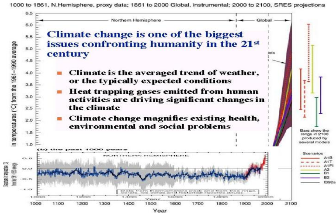
Figure 8.2 Past, present and future climate
