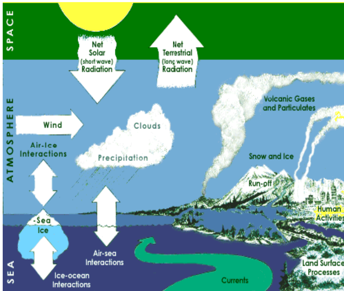
Figure 3.1 Major elements of the climate system [4] .
