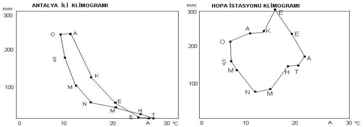
Figure 9.20 Climogram of some cities in Turkey
