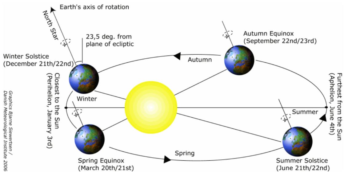
Figure 3.6 Earth trip around the sun through a year and seasons
