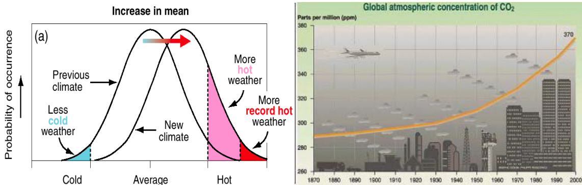
Figure 8.1 Shift in mean and CO2 concentration over time
