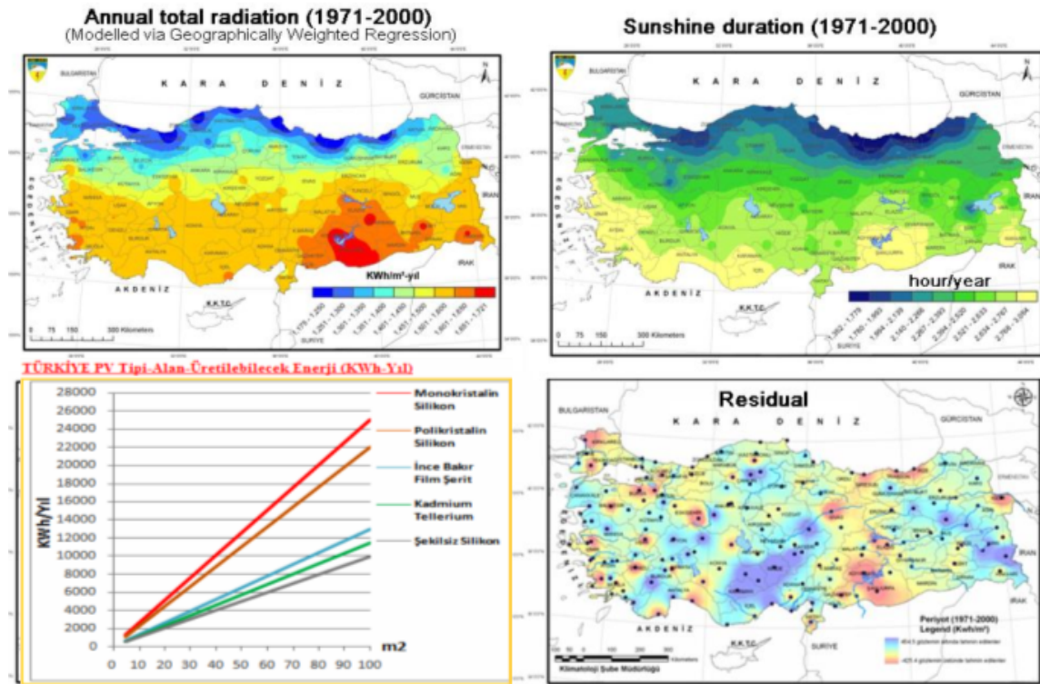
Figure 9.21 Solar energy atlas of Turkey
