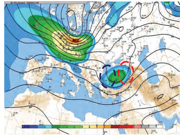
Figure-81 500 hPa chart (left) 23.09.2012, 00 UTC and 300 hPa jet stream (right) 22.09.2012, 12 UTC
