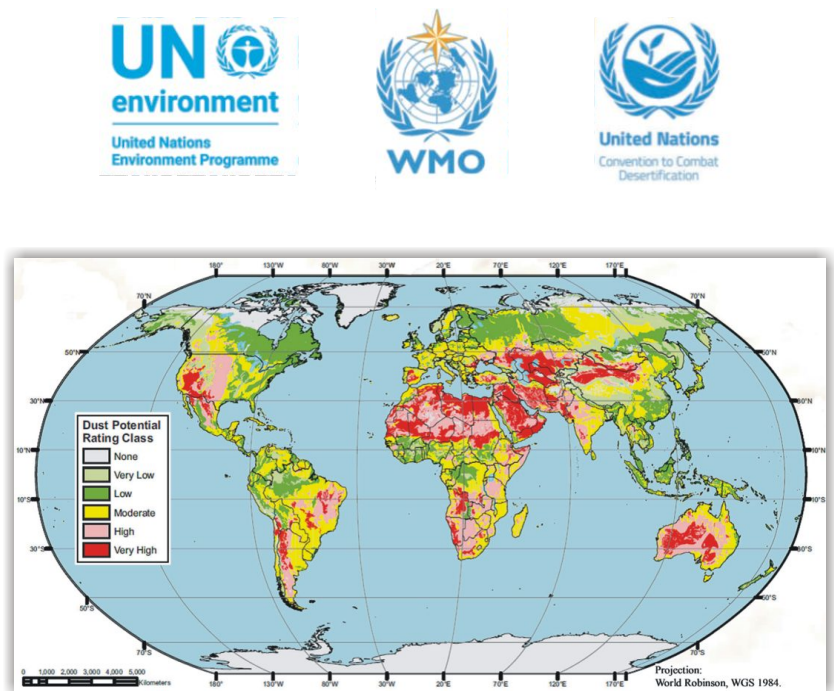
Figure 1. Global Dust Potential Map. Source: DTF (2013) [9]
