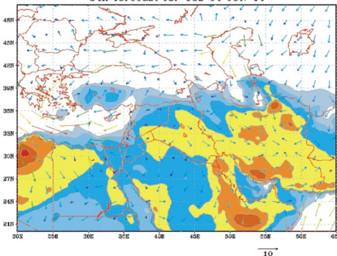
TMS/BSC-DREAM8b Surface Concentration ( \mu\text{g}/\text{m}^3 ) and Wind at 10m 54h forecast for 18z 04 JUN 14
